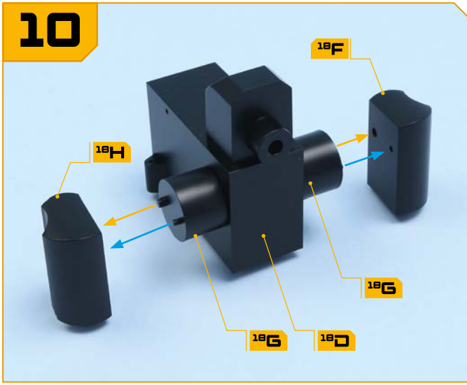
#018-10 Take the two connecting rings 18G and the video support 18D . Fit one of the rings on each side of the support. Note that the rings have different sized pegs: the smaller peg (circled) should be next to the edge of the support. These are push-fit connections.
